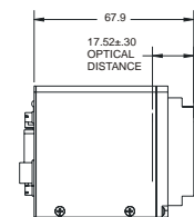
C- MOUNT CONFIGURATION
