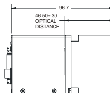
F- MOUNT CONFIGURATION
